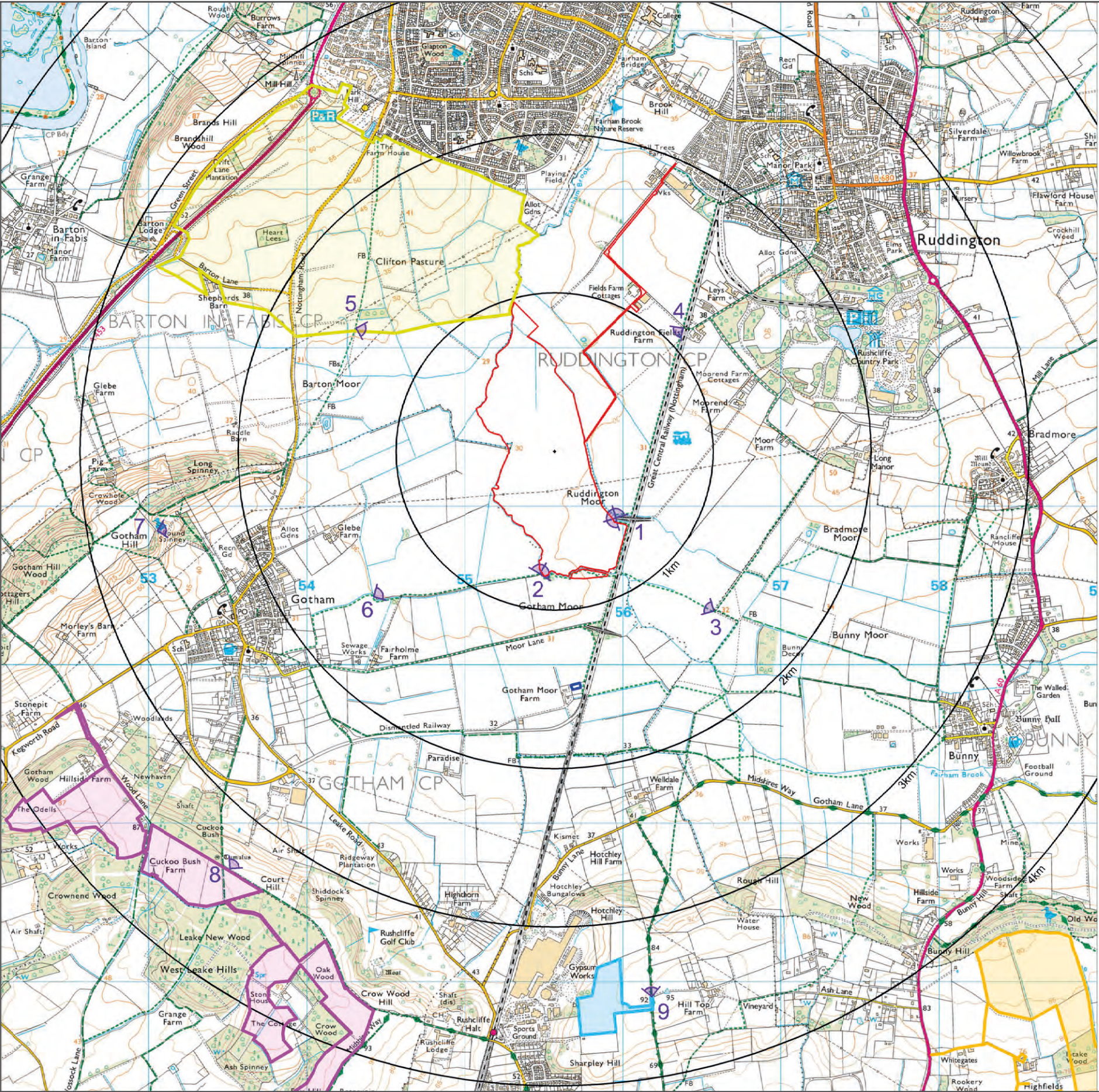
Figure 9.6: Permitted and Proposed Solar Farm Developments
