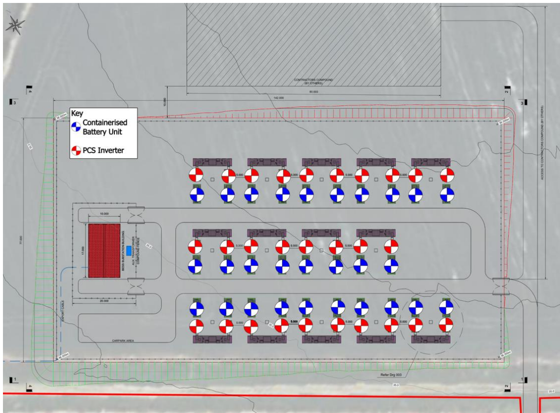
Figure 3: Proposed Layout of Six Oaks Renewable Energy Park Battery Storage Area
