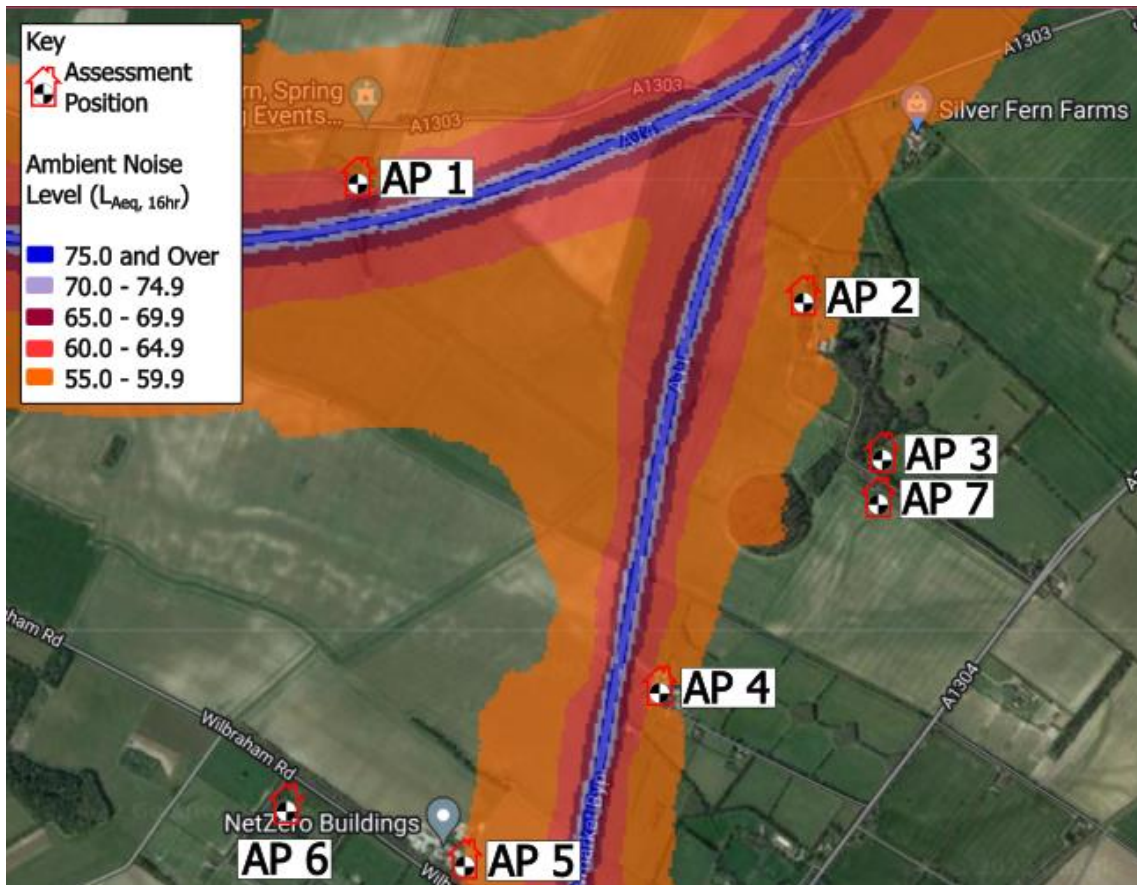
Figure 4: Daytime Noise Contour ( L_{Aeq,16hrs} ). The extrapolated APs are labelled.
