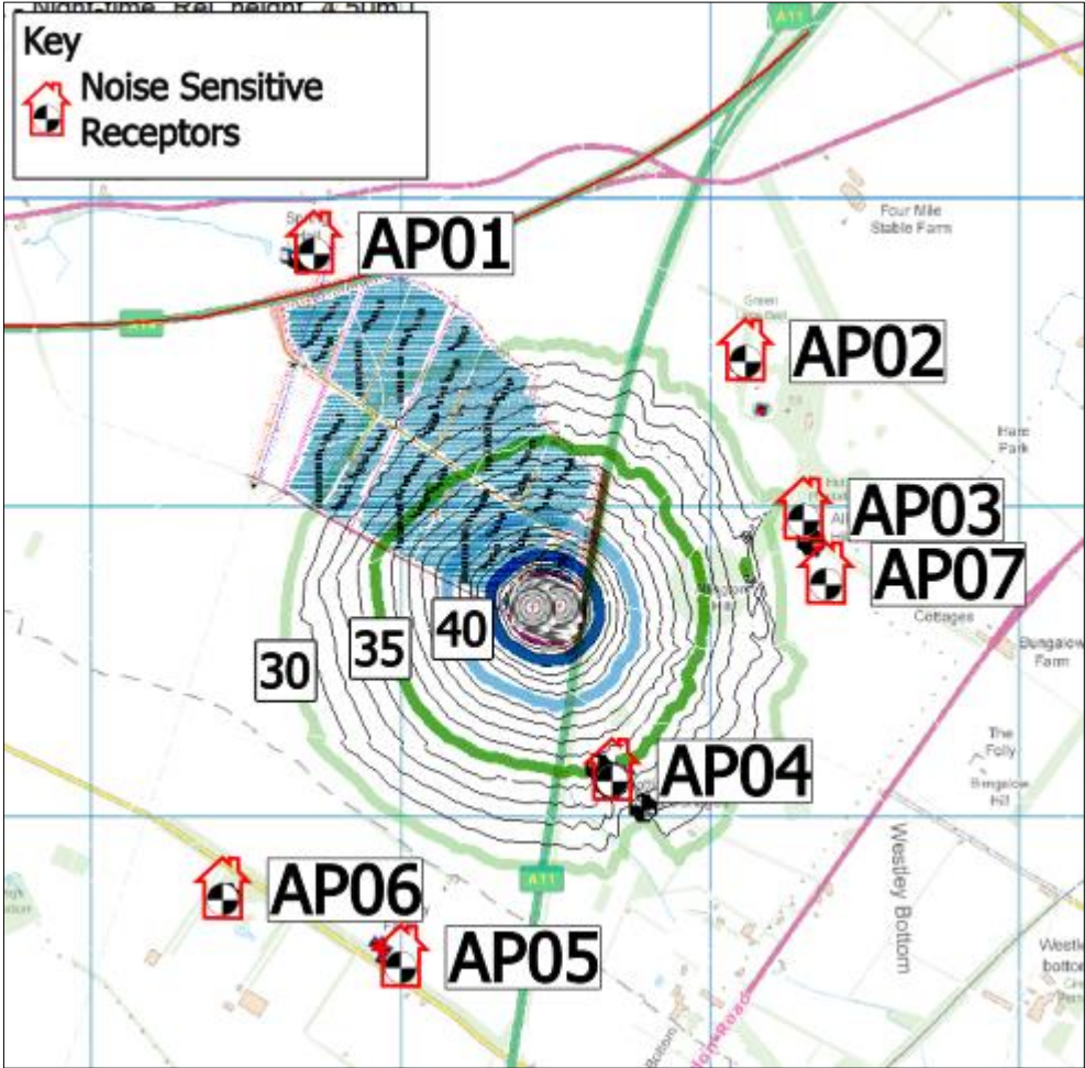
Figure 7: Indicative Night-time Noise Contour Plot, dB LAeq
