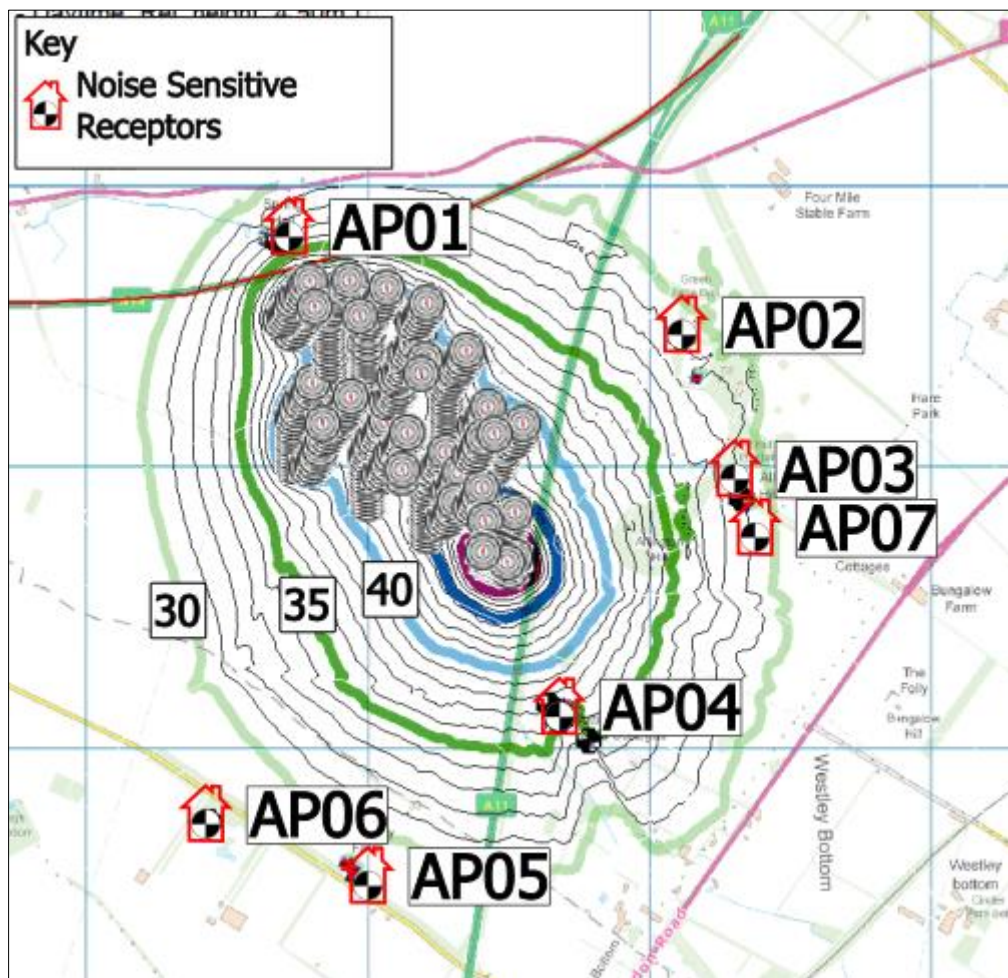
Figure 6: Indicative Daytime Operation Noise Contour Plot, dB L_{Aeq}
