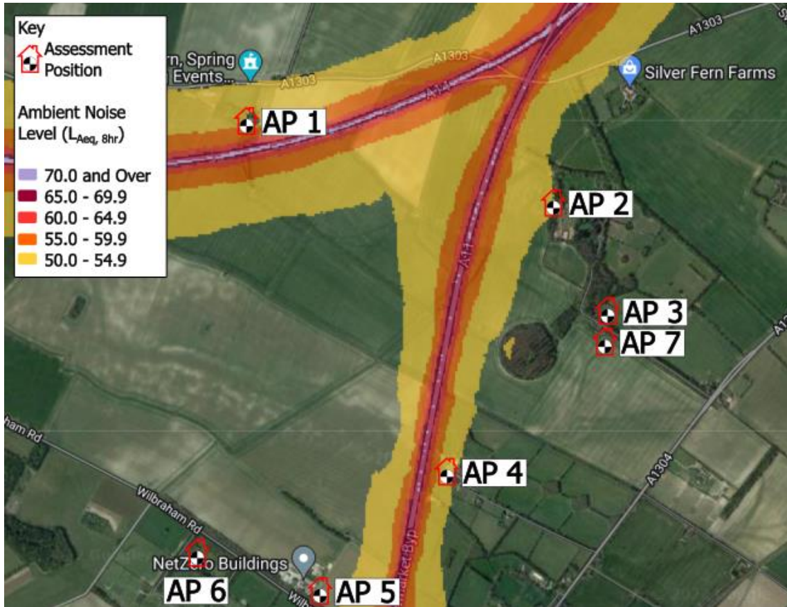
Figure 5: Night-time Noise Levels ( L_{Aeq,8hrs} ). The extrapolated APs are labelled.
